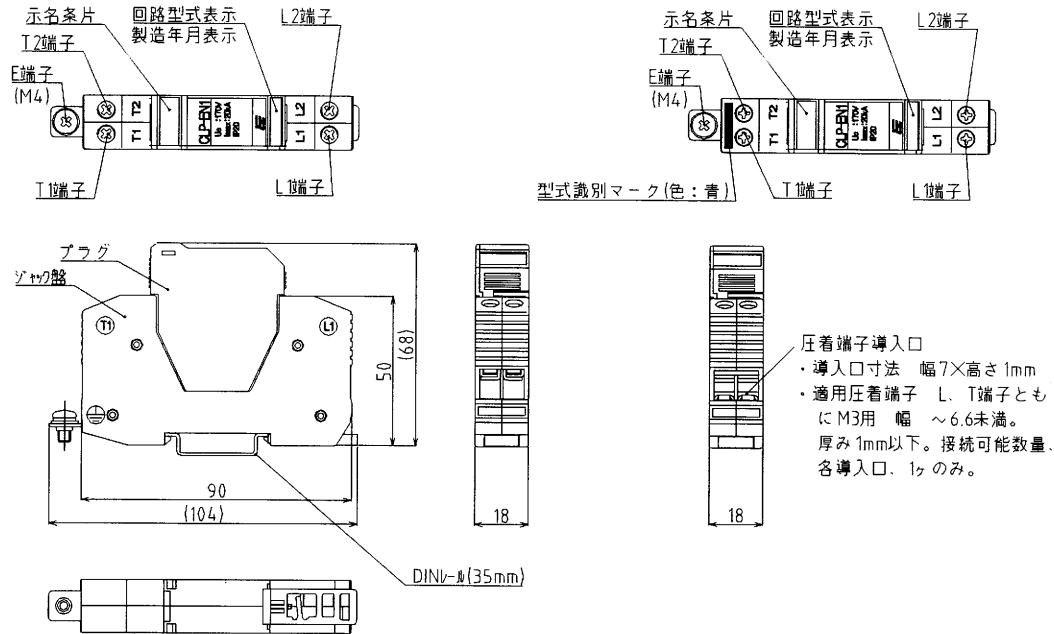
図1(図面はEN1形、右図:ねじ端子)
